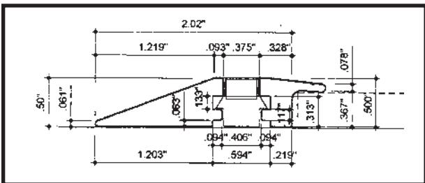
Carpet-to-Floor Extrusion CFE
