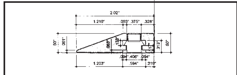
Floor-to-Wall Extrusion FWE
