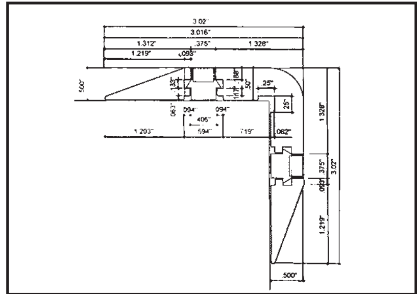
Floor-to-Wall Extrusion FWE
