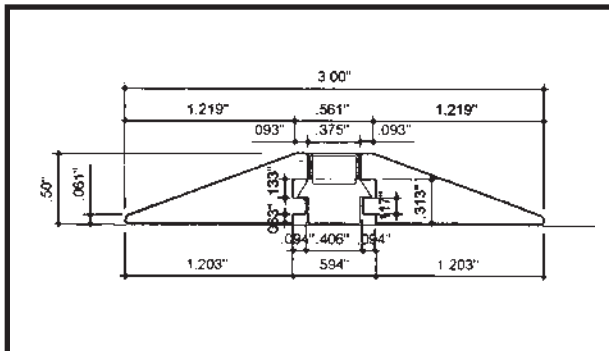
Carpet-to-Floor Extrusion CFE
