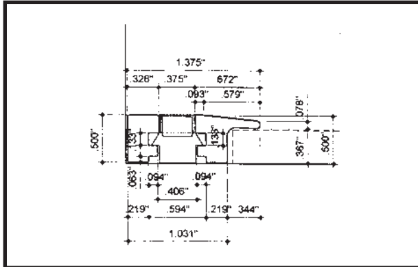
Floor-to-Floor Extrusion FFE
