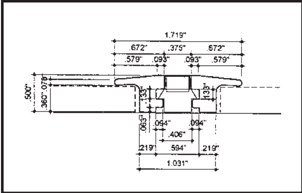
Carpet-to-Wall Extrusion CWE
