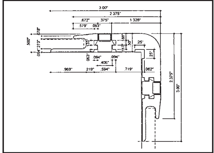
Floor-to-Floor Bullnose Extrusion FFBE
